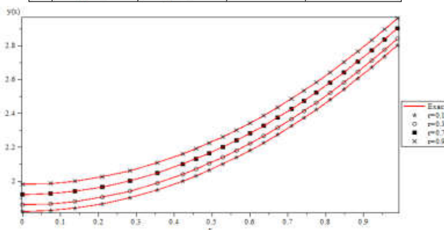
Fig. 1. Approximate solution of y(x,r) for r = 0.1, 0.3, 0.7, 0.9 of Example 1.
