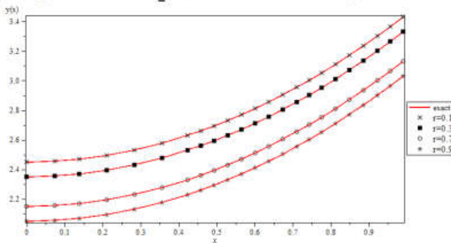
Fig. 2. Approximate solution of \bar{y}(x,r) for r = 0.1, 0.3, 0.7, 0.9 of Example 1.
