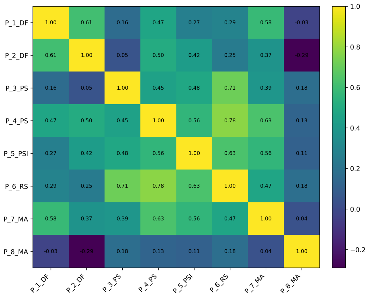
Figure 2. Correlation matrix of the eight questionnaire predictors
