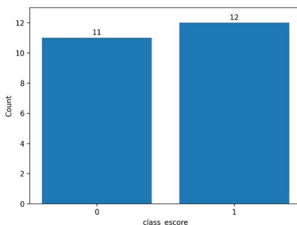
Figure 1. Binary outcome distribution
