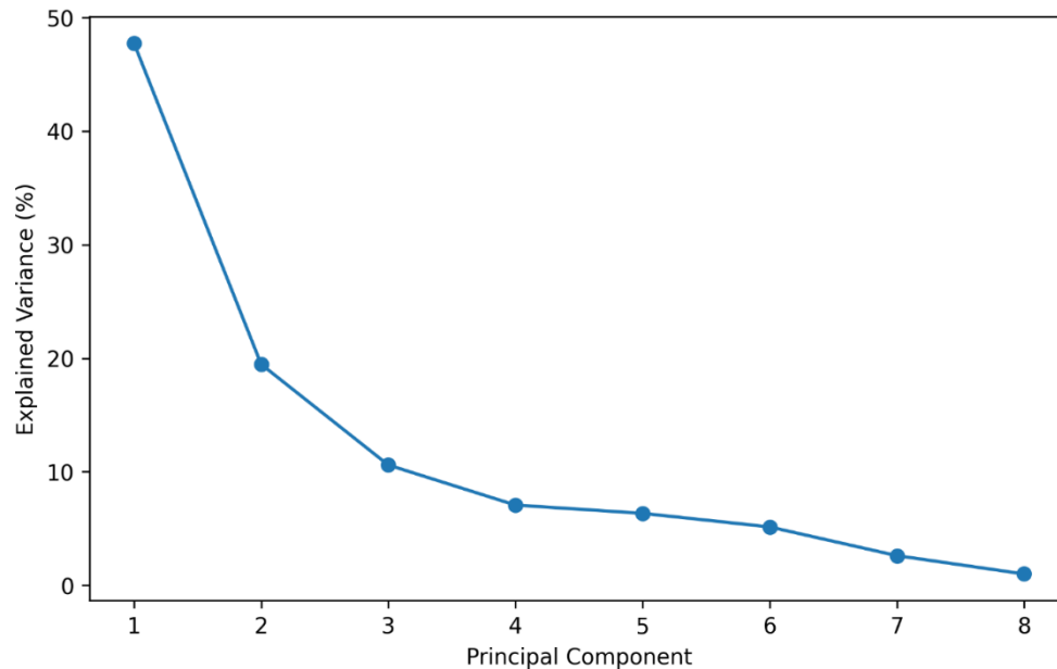
Figure 3. PCA scree plot and cumulative explained variance
