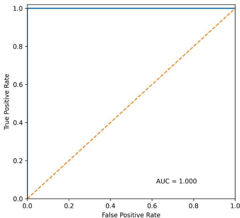
Figure 4. ROC curve for the PCA–Firth logistic regression model
